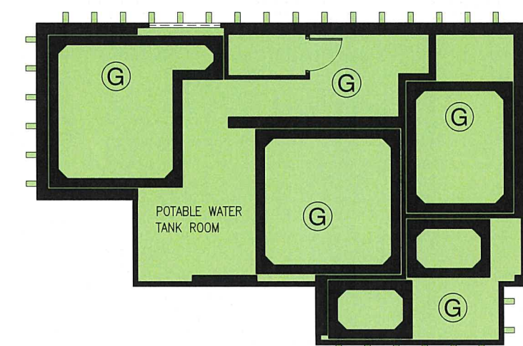
M & E FLOOR PLAN AT LEVEL 170.80
