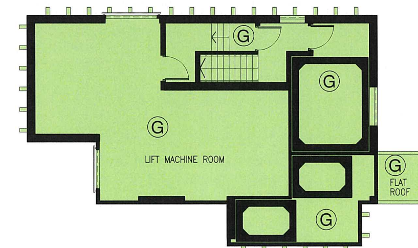
M & E FLOOR PLAN AT LEVEL 167.25
