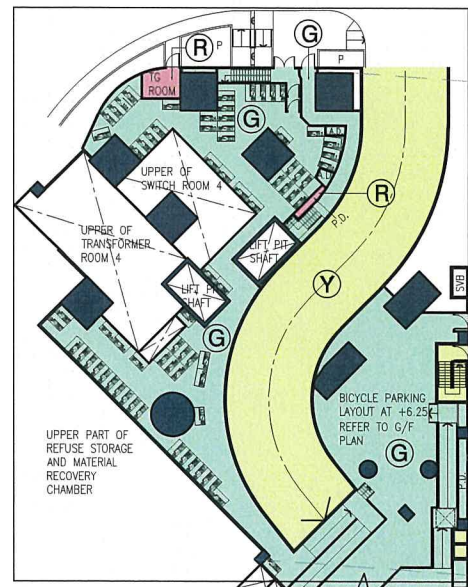
PART PLAN AT LEVEL 7.45
