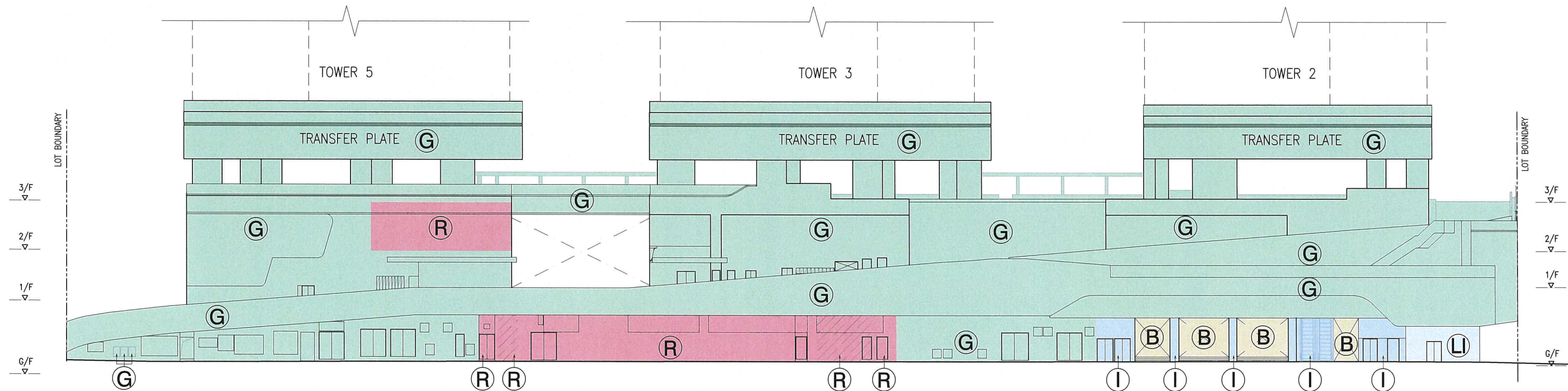
PODIUM SOUTH WEST ELEVATION C
