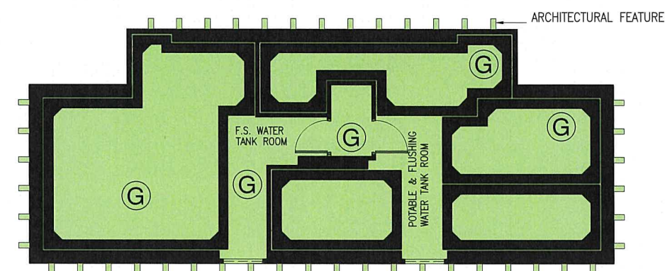
UPPER ROOF PLAN AT LEVEL 164.22
